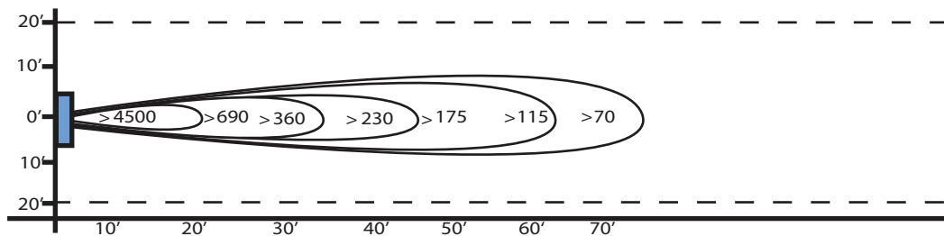
HVTC High Velocity Fan Air Flow Pattern
